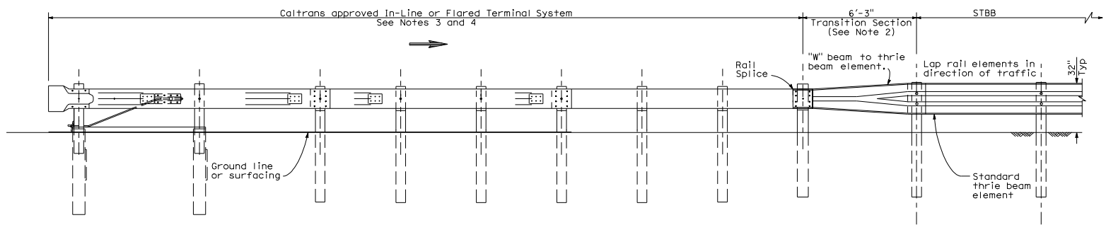
ELEVATION END TREATMENT FOR TRAFFIC APPROACH END OF SINGLE THRIE BEAM BARRIER
